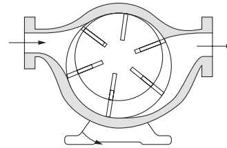
Vane pump
