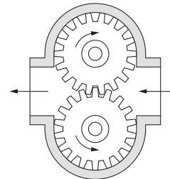
Gear pump
